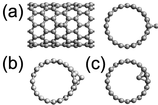
FIG. 1. Ball-and-stick representation of a (10,0) single-walled zigzag nanotube with a carbon adatom, as calculated by the DFTB method. (a) The adatom is above a bond parallel to the tube axis (top and side views). (b) The adatom is on top of a bond perpendicular to the tube axis (side view). (c) Adatom is inside the tube.
