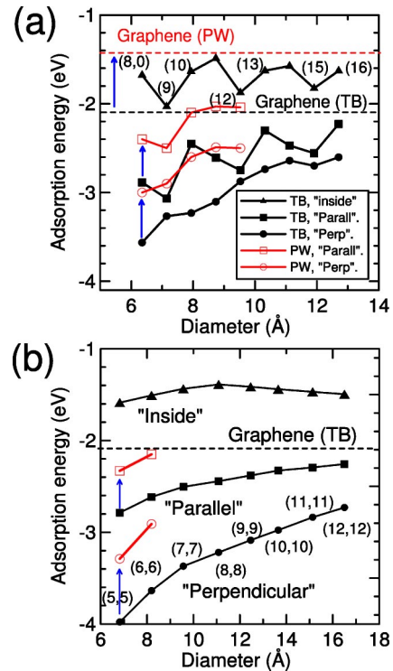
FIG. 2. (Color online) Adsorption energies of carbon adatoms on zigzag (a) and armchair (b) single-walled nanotubes as functions of tube diameters. The arrows visualize the relationship between the corresponding TB and PW results. The numbers stand for the tube chirality indices. The symbol legend for armchair tubes is the same as for zigzag ones.
