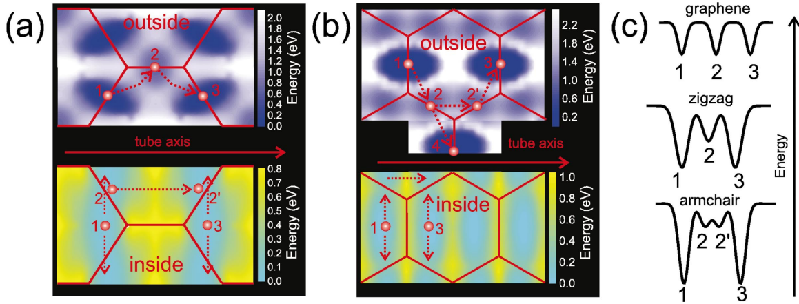
FIG. 3. (Color) Potential energy surface as a function of the adatom position on a zigzag (8,0) nanotube (a) and a (5,5) armchair SWNT (b) as calculated by the DFTB method. Circles stand for stable/metastable adatom positions, dotted lines show migration paths. Schematic energy diagrams for adatoms outside the tube (c).
