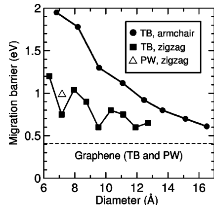
FIG. 4. Energy barrier for adatom migration on the outer surface of nanotubes as a function of nanotube diameters. The graphene migration barrier is the same in both PW and TB calculations.
