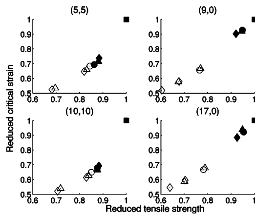
FIG. 4. Tensile strength and critical strain of nanotubes with defects. Filled symbols correspond to reconstructed vacancies and open symbols to nonreconstructed vacancies. Squares are the reference values for perfect tubes, circles stand for tubes with a monovacancy, triangles with a double vacancy and diamonds for tubes with a triple vacancy.
