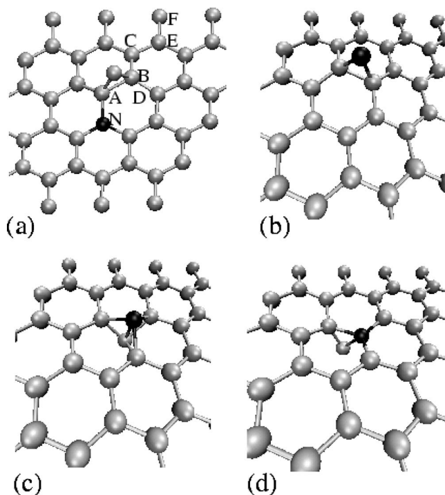
FIG. 4. (a) Graphene sheet with a substitutional N atom and a C adatom. Migration path (b) \Rightarrow (c) \Rightarrow (d) from a graphene layer with a N adatom (b) to a graphene with a substitutional N atom and a C adatom (d). The N atom “pushes” down one of the underlying C atoms and forms a “dumbbell” at the saddle point (c). The grey and black spheres represent C and N atoms, respectively.
