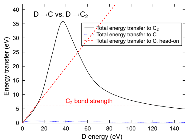
Fig. 3. Comparison of energy transfer from a D ion to the two atoms in a C dimer and a single C atom. The “total energy transfer to C” was calculated for the same lateral distance (impact parameter) from the ion to the C nucleus as in the dimer case. In the “head-on” case the impact parameter was zero.
