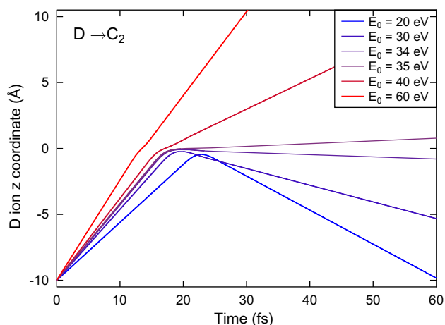
Fig. 4. z Coordinate of D atom while it collides with a C_2 dimer.
