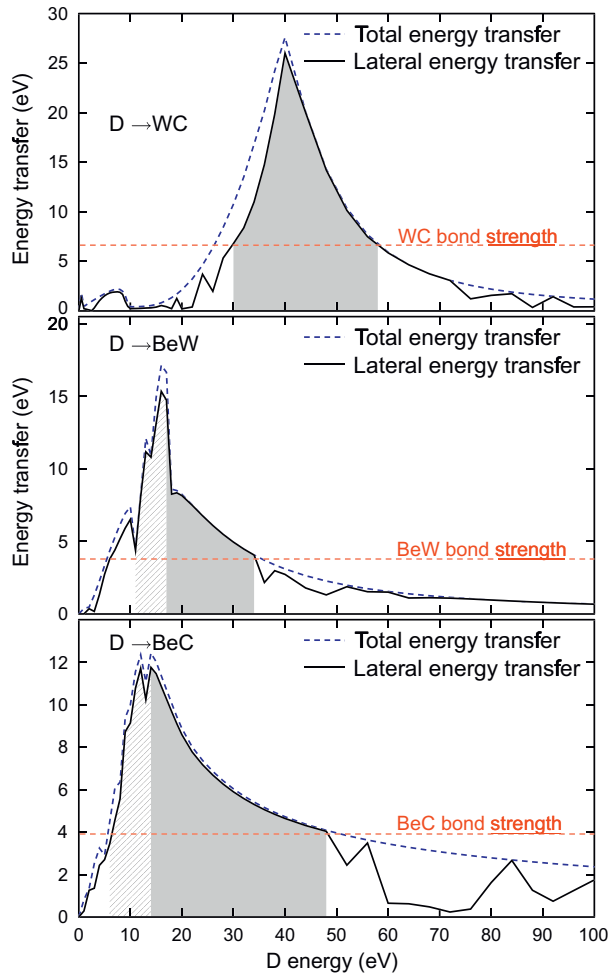
Fig. 7. As Fig. 2, but for the mixed dimers WC, BeW and BeC. The hashed area shows the energy interval where the dimer bond is broken, but the incoming D remains bonded to one of the atoms that was initially part of the dimer.
